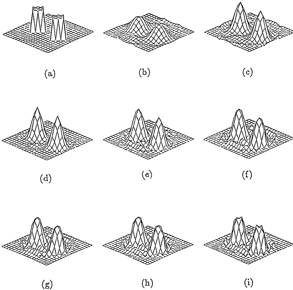
Figure 3.14. Reconstruction of a two-pulse distribution by using the distorted Born iterative method with operating frequency at 100 MHz. The peak value of the relative permittivity is 1.80. The diameter of the object is 3.0 meters. (a) is the original distribution. (b) is the result of the first-order approximation. (c) to (h) are the results from the second iteration to the seventh iteration. (i) is the final convergent solution after fifteen iterations.
