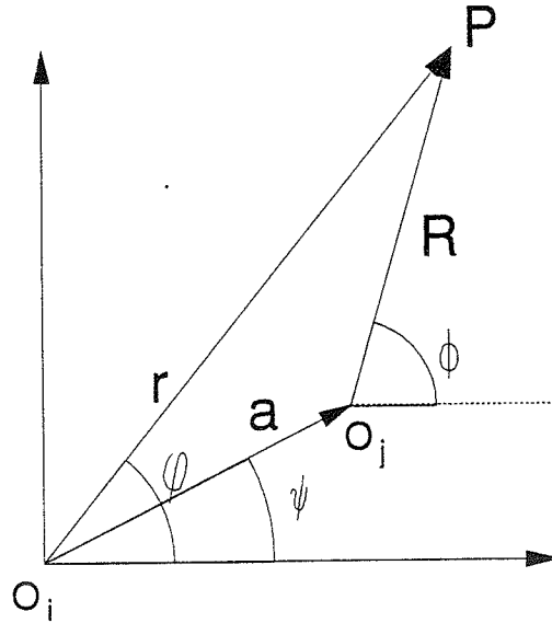
Figure A.1. Translation in the cylindrical coordinate systems.
