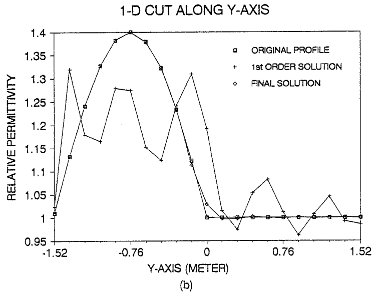
Figure 4.10. (a) is the 1-D cut of the reconstructed distribution shown in Figure 4.9 along the x -axis. (b) is the 1-D cut of the reconstructed distribution along the y -axis. The line with squares is for the original profile. The line with crosses is for the first-order solution, and the line with diamonds is for the final convergent solution.
