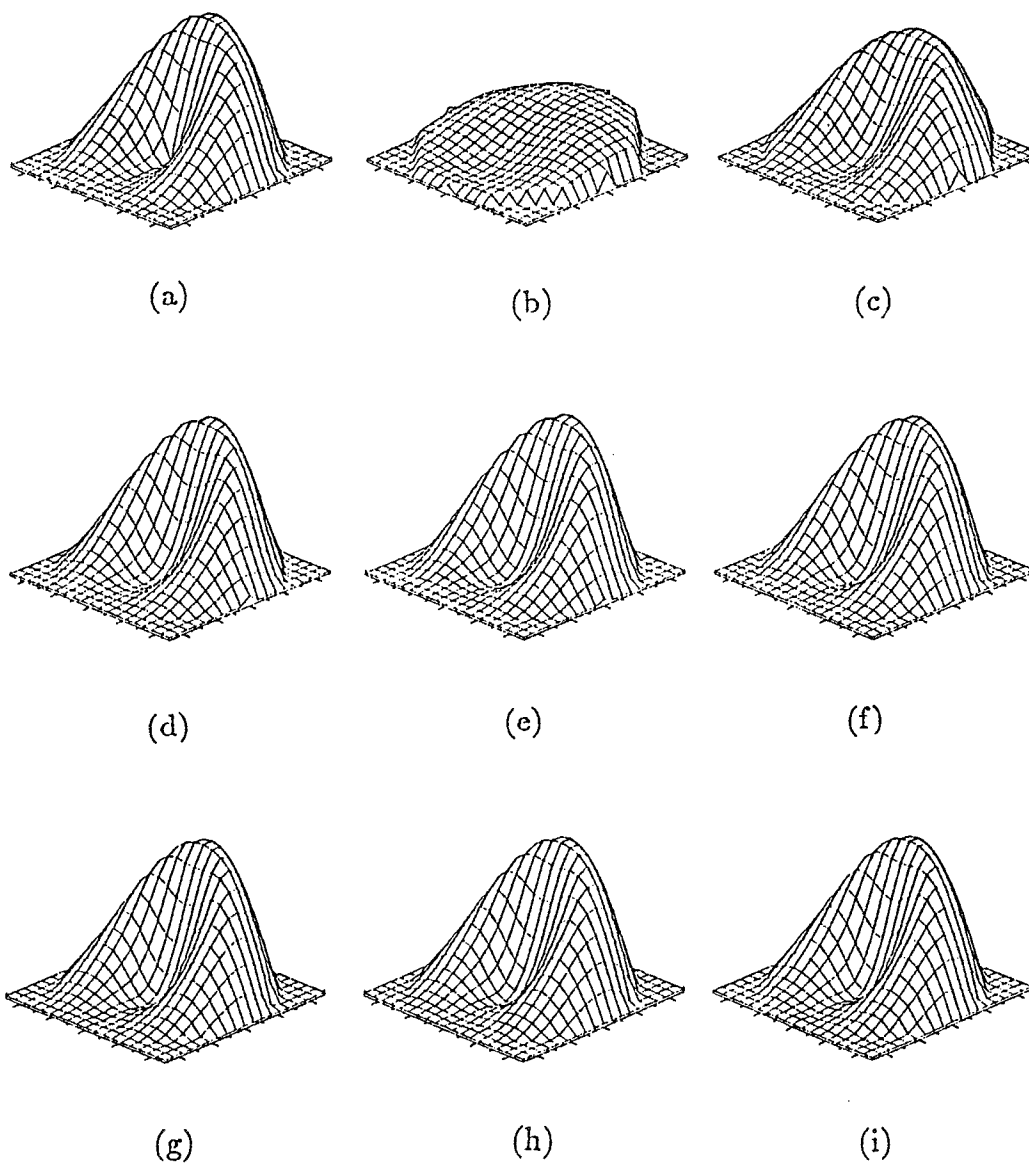
Figure 3.9. Reconstruction of an asymmetric distribution with operating frequency at 100 MHz. The peak value of the relative permittivity is 1.8. The diameter of the object is 3.0 meters. (a) is the original distribution. (b) is the result of the first-order approximation. (c) to (h) are the results from the second iteration to the seventh iteration. (i) is the final convergent solution after twenty-five iterations.
