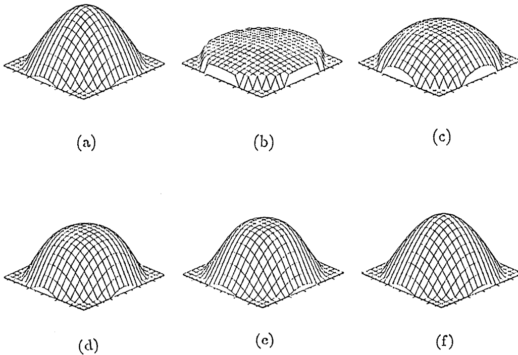
Figure 3.12. Reconstruction of a sinelike permittivity distribution by using the Born iterative method with operating frequency at 100 MHz. The peak value of the relative permittivity is 1.80. The diameter of the object is 3.0 meters. (a) is the original distribution. (b) is the result of the first-order approximation. (c) to (e) are the results from the second iteration to the fourth iteration. (f) is the final convergent solution after fifteen iterations.
