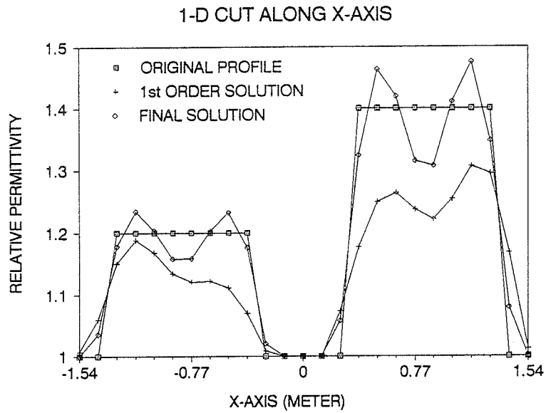
Figure 4.13. 1-D cut of the reconstructed distribution shown in Figure 4.12 along the x -axis. The line with squares is for the original profile. The line with crosses is for the first-order solution, and the line with diamonds is for the final convergent solution.
