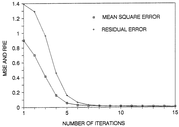
Figure 4.5. The relative MSE (Mean Square Error) and the RRE (Relative Residual Error) of the reconstructed permittivity distribution shown in Figure 4.3 as a function of the iteration steps.
