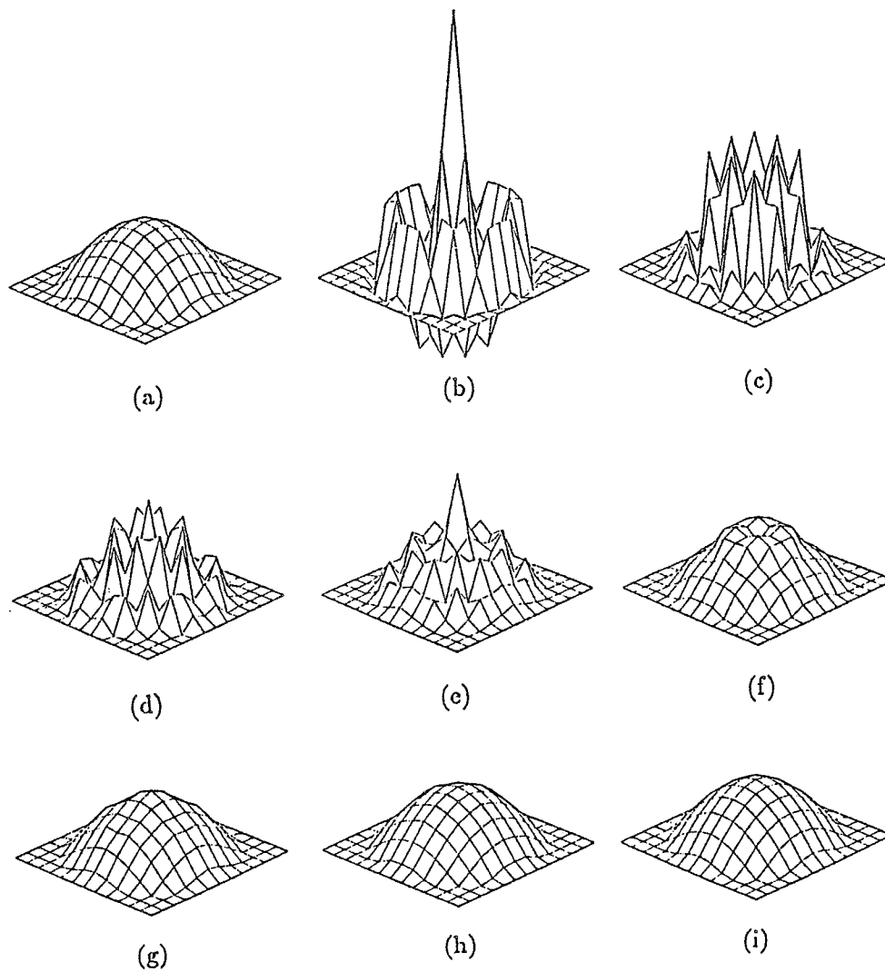
Figure 3.3. Reconstruction of a sinelike permittivity distribution with operating frequency at 100 MHz. The peak value of the relative permittivity is 1.80. The diameter of the object is 1\lambda . (a) is the original distribution. (b) is the result of the first-order approximation. (c) to (h) are the results from the second iteration to the seventh iteration. (i) is the final convergent solution after eight iterations.
