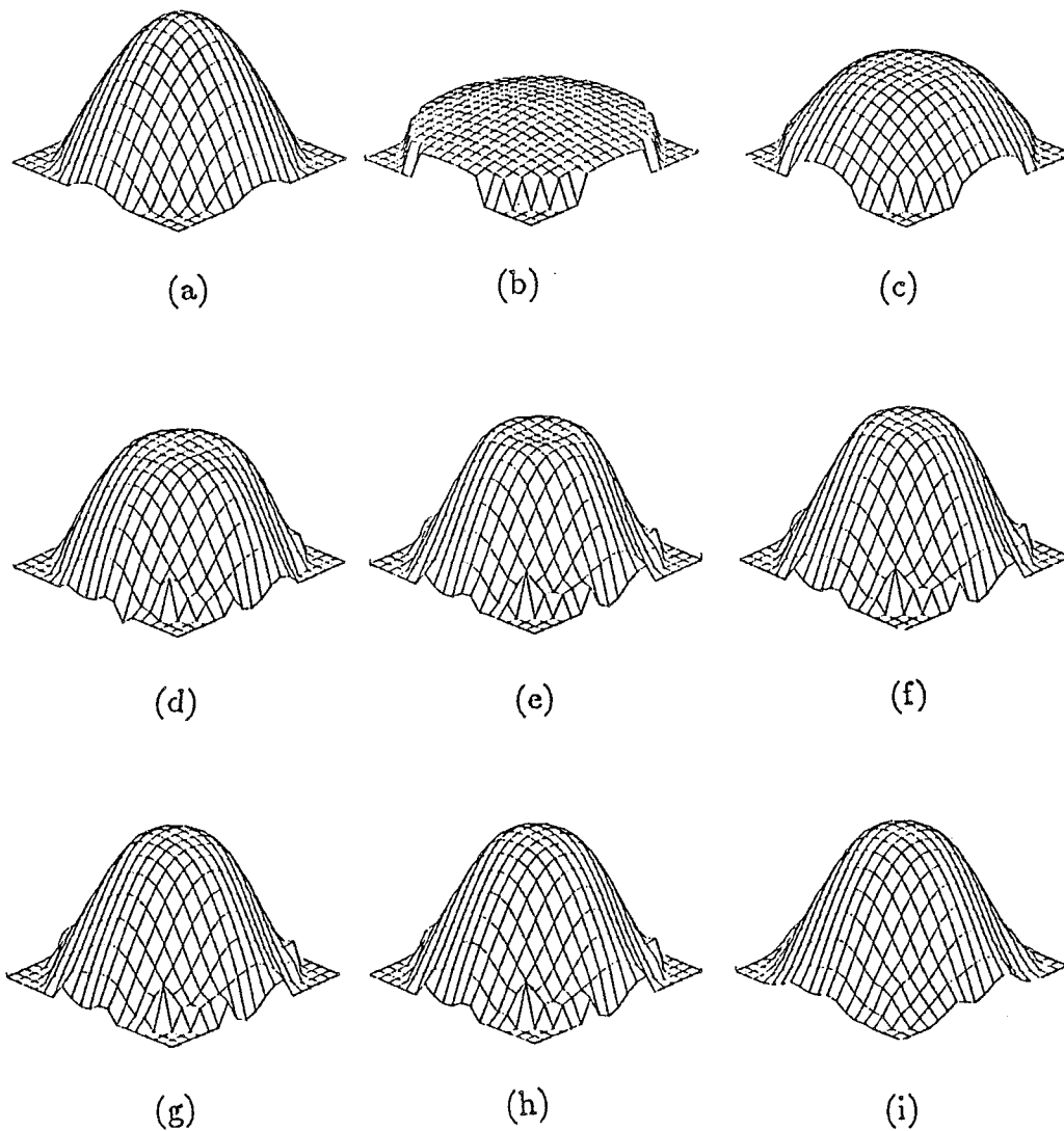
Figure 18. Reconstruction by using the Born iterative method for the same problem given in Figure 17. (a) is the original distribution. (b) is the result of the first-order approximation. (c) to (g) are the results from the second iteration to the sixth iteration. (h) is the convergent distribution after the fifteen iterations. (i) the reconstructed distribution after operating the filter function on (h).
