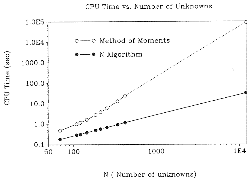
Figure 2.11. Comparison of the computer times for the fast recursive algorithm and the method of moments.
