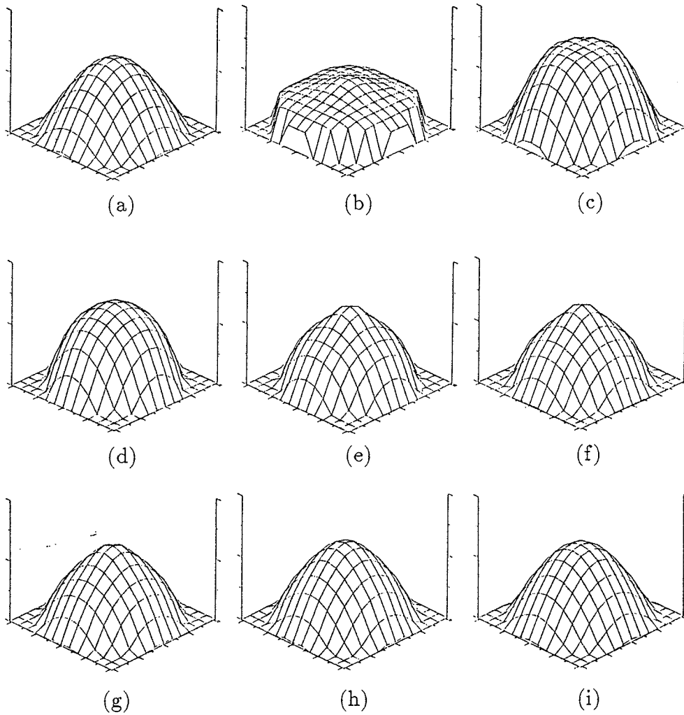
Figure 3.25. Evolution of the convergence of the imaginary part of the reconstructed complex permittivity distribution by using the distorted Born iterative method with operating frequency at 100 MHz. The peak value of the imaginary part of the relative permittivity is 0.6. The diameter of the object is 3.0 meters. (a) is the original distribution. (b) is the result of the first-order approximation. (c) to (h) are the results from the second iteration to the seventh iteration. (i) is the final convergent solution after twenty iterations.
