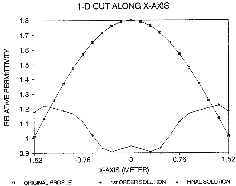
Figure 4.7. 1-D cut of the reconstructed distribution shown in Figure 4.6 along the x -axis. The line with squares is for the original profile. The line with crosses is for the first-order solution, and the line with diamonds is for the final convergent solution.
