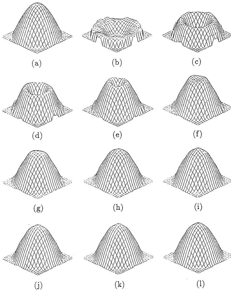
Figure 4.3. Reconstruction of a sinelike permittivity distribution using the distorted Born iterative algorithm without the boosting procedure with operating frequency at 200 MHz. The peak value of the relative permittivity is 1.8. The diameter of the object is about 2\lambda . (a) is the original distribution. (b) is the result of the first-order Born approximation. (c) to (k) are the results from the second iteration to the tenth iteration. (l) is the final convergent solution after 15 iterations.
