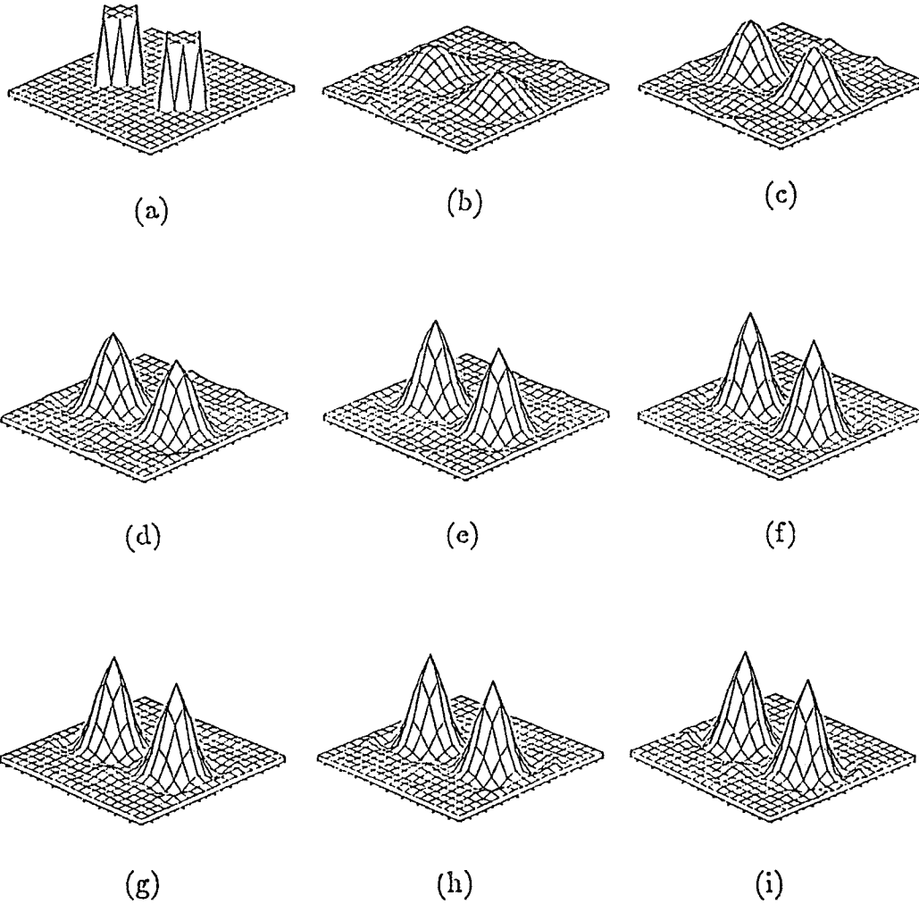
Figure 3.15. Reconstruction of a two-pulse distribution by using the Born iterative method with operating frequency at 100 MHz. The peak value of the relative permittivity is 1.80. The diameter of the object is 3.0 meters. (a) is the original distribution. (b) is the result of the first-order approximation. (c) to (h) are the results from the second iteration to the seventh iteration. (i) is the final convergent solution after fifteen iterations.
