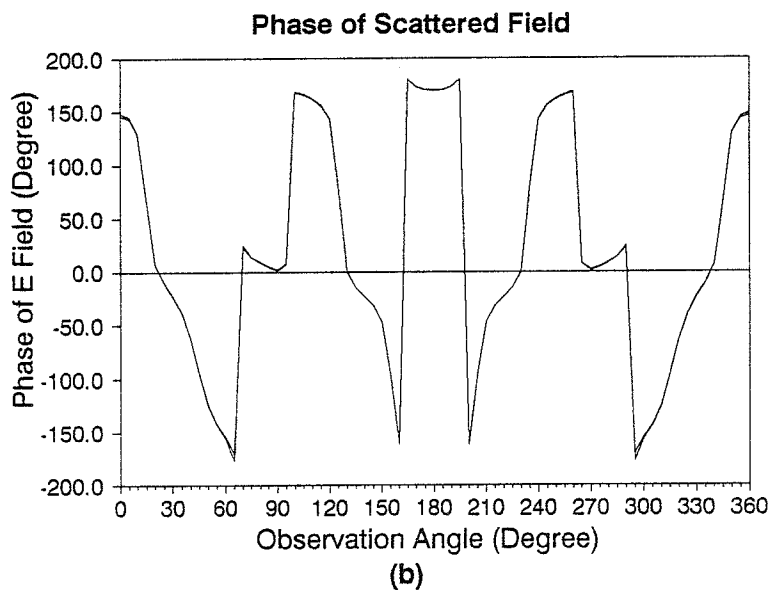
Figure 2.6. Comparison of the scattered fields by using the aggregate \tau matrix method and the method of moments. (a) Amplitude of the scattered field as a function of the observation angles. (b) Phase of the scattered field as a function of the observation angles.
