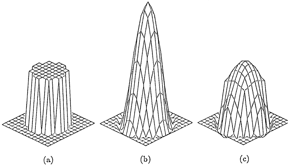
Figure 3.6. Reconstruction of a step permittivity distribution with operating frequency at 10 MHz. The contrast of the relative permittivity is 1:11. The diameter of the object is 0.1\lambda . (a) is the original distribution. (b) is the result of the first-order approximation. (c) is the final convergent solution after five iterations.
