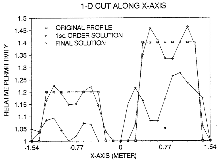
Figure 4.19. 1-D cut of the reconstructed distribution shown in Figure 4.18 along the x -axis. The line with squares is for the original profile. The line with crosses is for the first-order solution, and the line with diamonds is for the final convergent solution.
