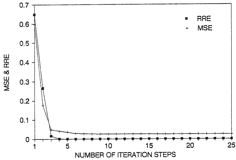
Figure 3.10. The relative MSE (Mean Square Error) and the RRE (Relative Residual Error) of the reconstructed permittivity distribution in Figure 3.9 as a function of the iteration steps.
