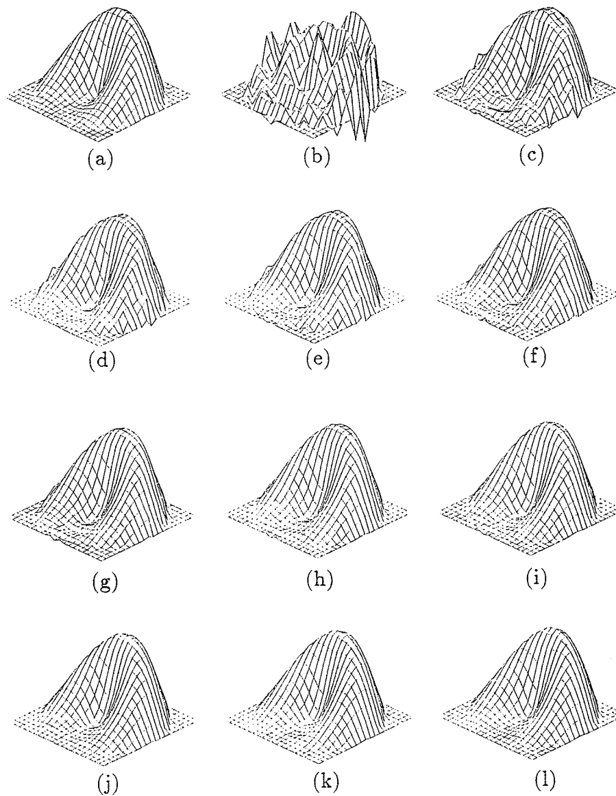
Figure 4.9. Reconstruction of an asymmetric permittivity distribution using the distorted Born iterative algorithm with the boosting procedure with operating frequency at 200 MHz in well-to-well tomography. The peak value of the relative permittivity is 1.4. The diameter of the object is about 2\lambda . (a) is the original distribution. (b) is the first-order Born solution. (c) to (k) are the results from the second iteration to the tenth iteration. (l) is the final convergent solution after 20 iterations.
