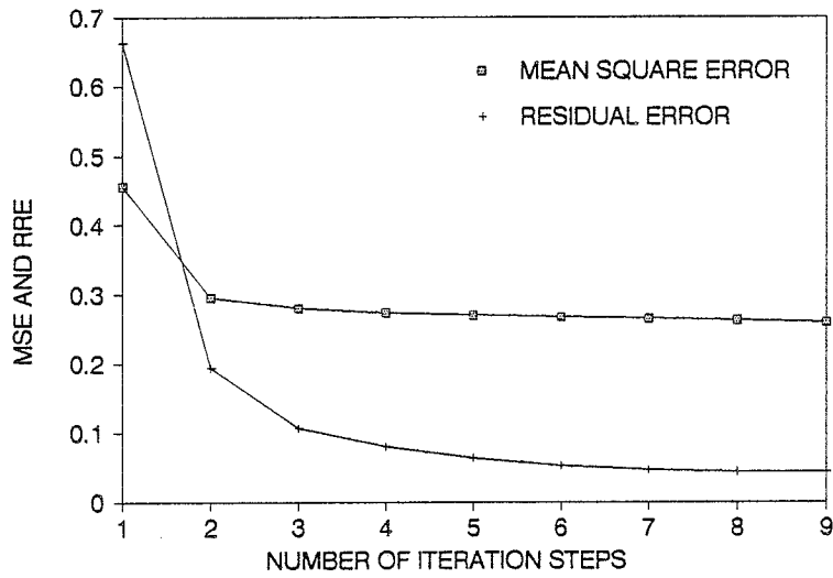
Figure 4.14. The relative MSE (Mean Square Error) and the RRE (Relative Residual Error) of the reconstructed permittivity distribution shown in Figure 4.12 as a function of the iteration steps.
