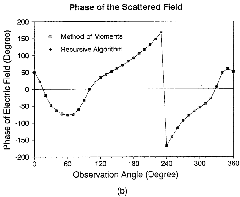
Figure 2.7. Comparison of the solutions from the method of moments and the fast recursive algorithm for an inhomogeneous dielectric scatterer. (a) Amplitude of the scattered field versus observation angle \phi . (b) Phase of the scattered field versus observation angle \phi .
