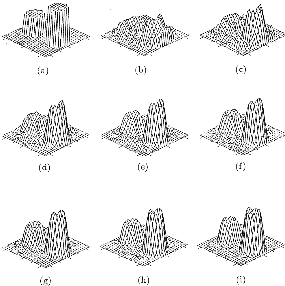
Figure 4.18. Reconstruction of a two-pulse permittivity distribution using the distorted Born iterative algorithm in subsurface detection with operating frequency at 200 MHz. The heights of the pulses are 1.2 and 1.4, respectively. The width of the pulses is about 0.65\lambda . The separation between the two pulses is about 0.42\lambda . (a) is the original distribution. (b) is the result of the first-order Born approximation. (c) to (h) are the results from the second iteration to the seventh iteration. (i) is the final convergent solution after 20 iterations.
