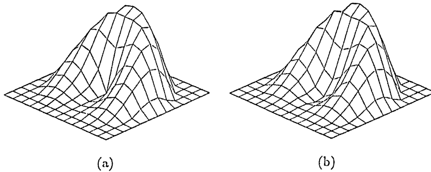
Figure 3.7. Reconstruction of an axially asymmetric permittivity distribution with operating frequency at 100 MHz. The peak value of the relative permittivity is 1.80. The diameter of the object is 1\lambda . (a) is the original distribution. (b) is the final convergent solution after six iterations.
