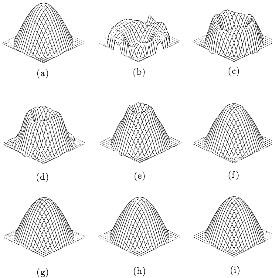
Figure 4.6. Reconstruction of a sinelike permittivity distribution using the distorted Born iterative algorithm with the boosting procedure with operating frequency at 200 MHz. The peak value of the relative permittivity is 1.8. The diameter of the object is about 2\lambda . (a) is the original distribution. (b) is the result of the first-order Born approximation. (c) to (h) are the results from the second iteration to the seventh iteration. (i) is the final convergent solution after 15 iterations.
