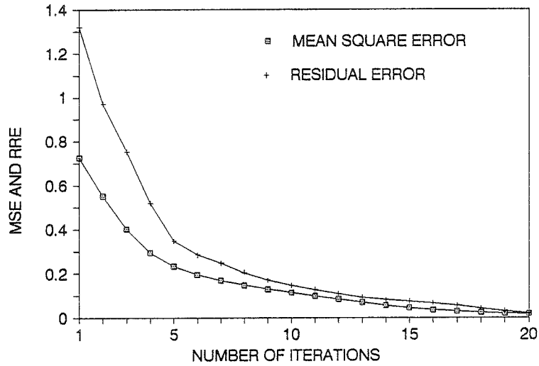
Figure 4.17. The relative MSE (Mean Square Error) and the RRE (Relative Residual Error) of the reconstructed permittivity distribution shown in Figure 4.15 as a function of the iteration steps.
