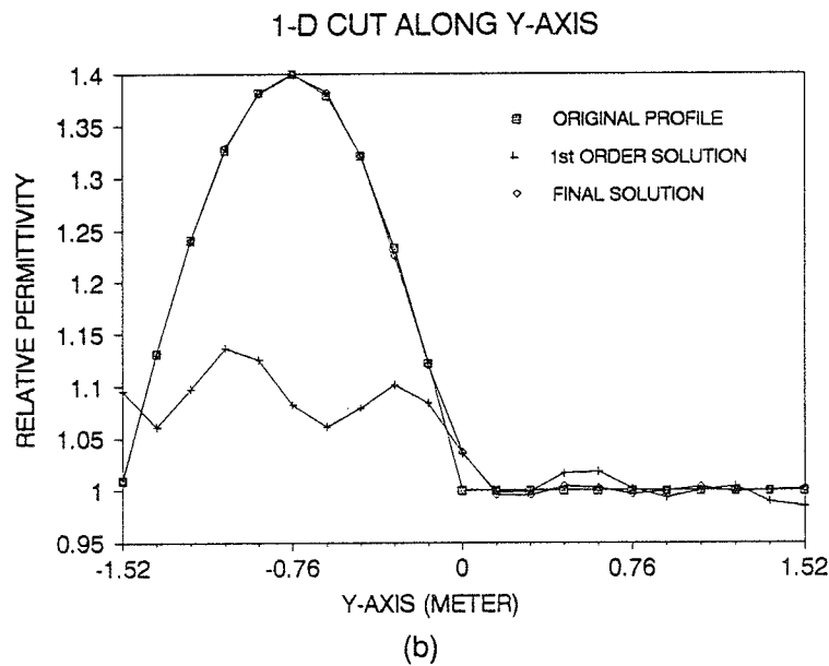
Figure 4.16. (a) is the 1-D cut of the reconstructed distribution shown in Figure 4.15 along the x -axis. (b) is the 1-D cut of the reconstructed distribution along the y -axis. The line with squares is for the original profile. The line with crosses is for the first-order solution, and the line with diamonds is for the final convergent solution.
