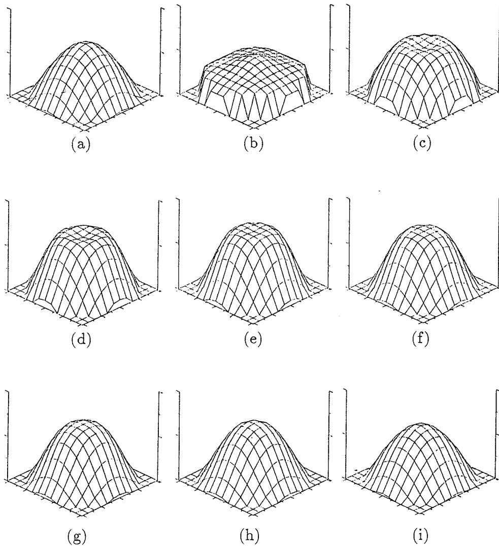
Figure 3.27. Evolution of the convergence of the imaginary part of the reconstructed complex permittivity distribution by using the Born iterative method with operating frequency at 100 MHz. The peak value of the imaginary part of the relative permittivity is 0.6. The diameter of the object is 3.0 meters. (a) is the original distribution. (b) is the result of the first-order approximation. (c) to (h) are the results from the second iteration to the seventh iteration. (i) is the final convergent solution after twenty iterations.
