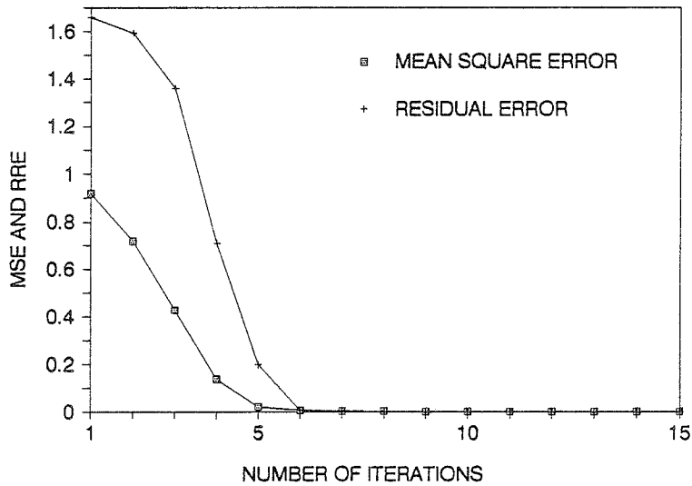
Figure 4.8. The relative MSE (Mean Square Error) and the RRE (Relative Residual Error) of the reconstructed permittivity distribution shown in Figure 4.6 as a function of the iteration steps.
