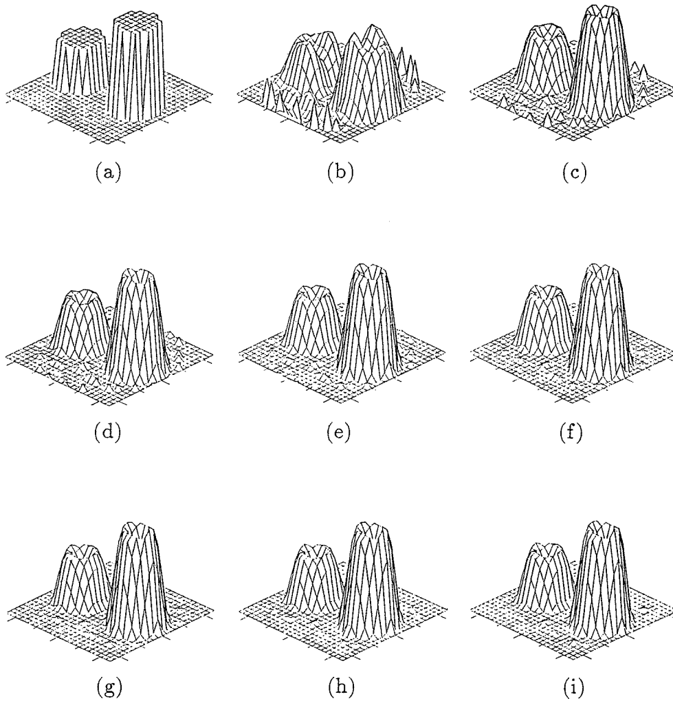
Figure 4.12. Reconstruction of a two-pulse permittivity distribution using the distorted Born iterative algorithm in well-to-well tomography with operating frequency at 200 MHz. The heights of the pulses are 1.2 and 1.4, respectively. The width of the pulses is about 0.65\lambda . The separation between the two pulses is about 0.42\lambda . (a) is the original distribution. (b) is the result of the first-order Born approximation. (c) to (k) are the results from the second iteration to the tenth iteration. (l) is the final convergent solution after 20 iterations.
