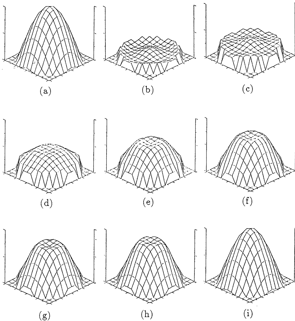
Figure 3.26. Evolution of the convergence of the real part of the reconstructed complex permittivity distribution by using the Born iterative method with operating frequency at 100 MHz. The peak value of the real part of the relative permittivity is 0.6. The diameter of the object is 3.0 meters. (a) is the original distribution. (b) is the result of the first-order approximation. (c) to (h) are the results from the second iteration to the seventh iteration. (i) is the final convergent solution after twenty iterations.
