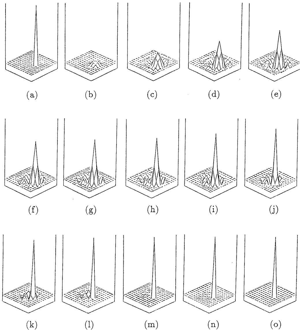
Figure 3.22. Reconstruction of a single-pixel pulse distribution by using the distorted Born iterative method with operating frequency at 100 MHz. The contrast of the relative permittivity is 1:11. The diameter of the reconstructed area is 3.0 meters. (a) is the original distribution. (b) is the result of the first-order approximation. (c) to (n) are the results from the second iteration to the thirteenth iteration. (o) is the final convergent solution after twenty iterations.
