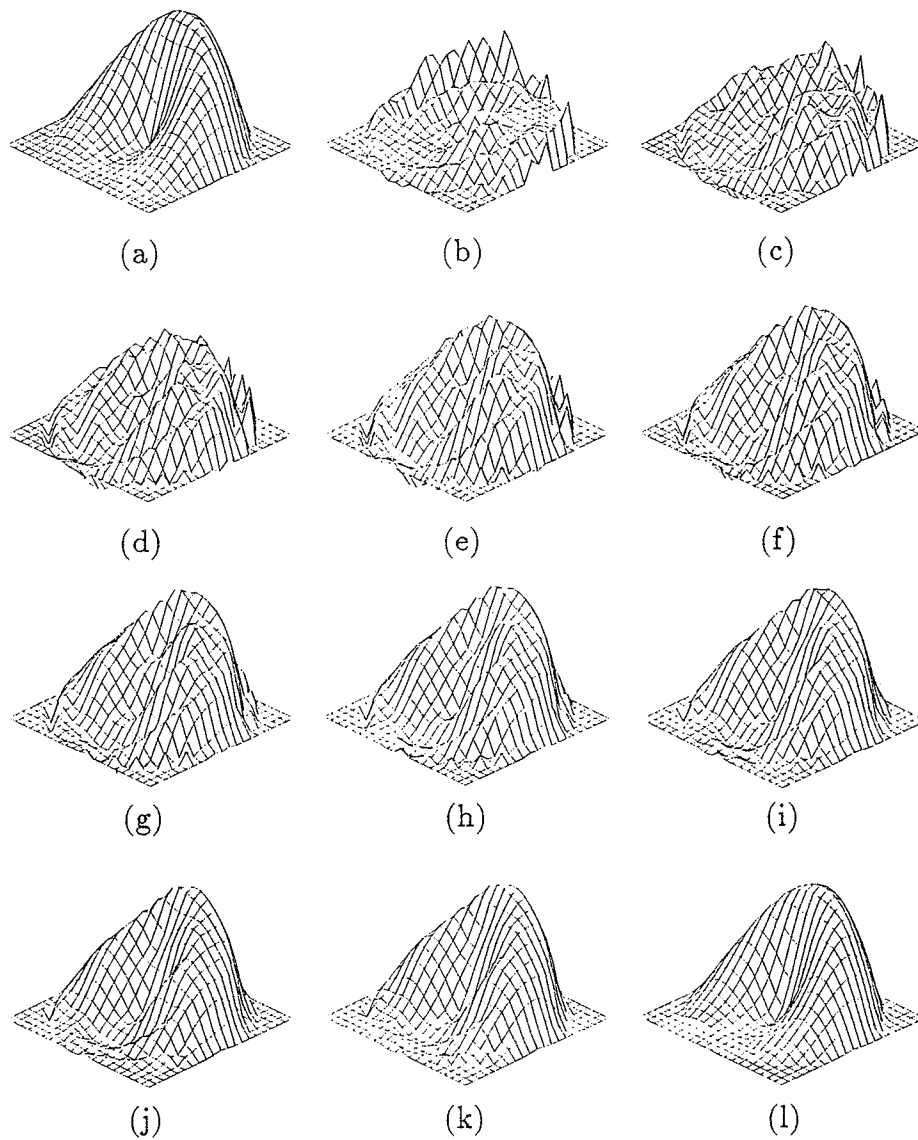
Figure 4.15. Reconstruction of an asymmetric permittivity distribution using the distorted Born iterative algorithm with the boosting procedure with operating frequency at 200 MHz in a subsurface detection problem. The peak value of the relative permittivity is 1.4. The diameter of the object is about 2\lambda . (a) is the original distribution. (b) is the first-order Born solution. (c) to (k) are the results from the second iteration to the tenth iteration. (l) is the final convergent solution after 20 iterations.
