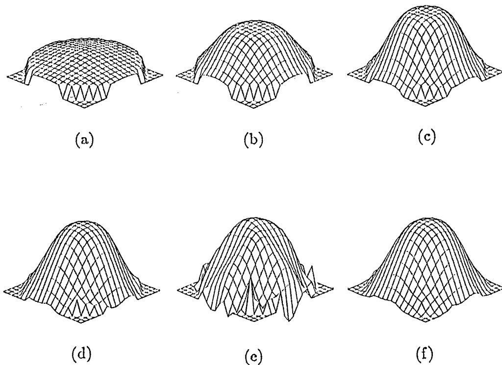
Figure 17. Reconstruction of a sinelike permittivity distribution with a 25 dB signal-to-noise ratio in the measurement field by using the distorted Born iterative method with operating frequency at 100 MHz. The peak value of the relative permittivity is 1.80. The diameter of the object is 1\lambda . (a) is the original distribution. (b) is the result of the first-order approximation. (c) to (e) are the results from the second iteration to the fourth iteration. (f) is the final distribution after operating the filter function on (d).
