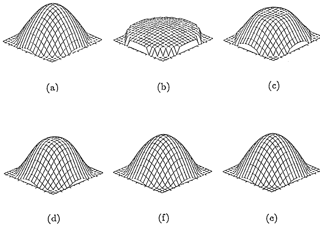
Figure 3.11. Reconstruction of a sinelike permittivity distribution by using the distorted Born iterative method with operating frequency at 100 MHz. The peak value of the relative permittivity is 1.80. The diameter of the object is 3.0 meters. (a) is the original distribution. (b) is the result of the first-order approximation. (c) to (f) are the results from the second iteration to the fourth iteration. (e) is the final convergent solution after fifteen iterations.
