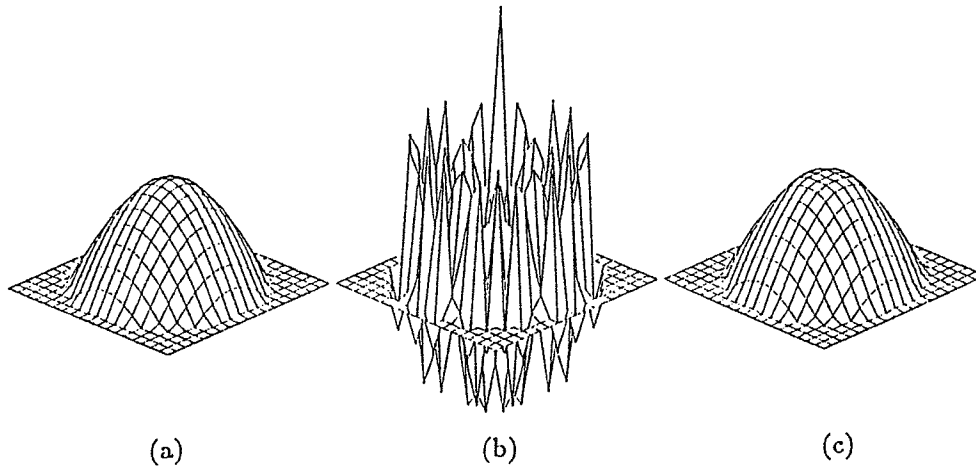
Figure 3.4. Reconstruction of a sinelike permittivity distribution with operating frequency at 200 MHz. The peak value of the relative permittivity is 1.80. The diameter of the object is 2\lambda . (a) is the original distribution. (b) is the result of the first-order approximation. (c) is the final convergent solution after twelve iterations.
