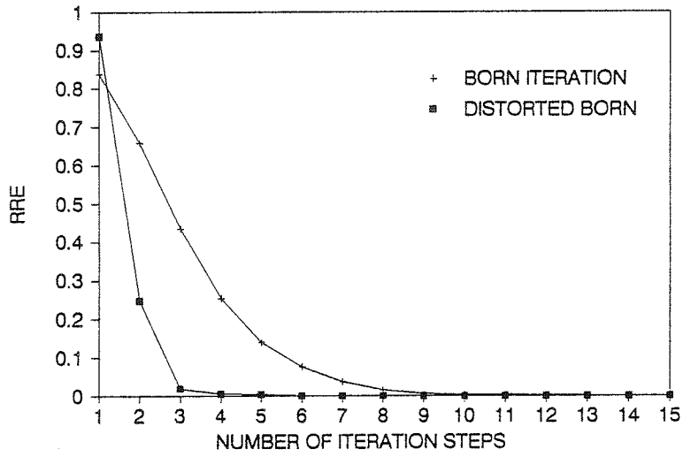
Figure 3.16. The RRE (Relative Residual Error) of the reconstructed permittivity distribution in Figures 3.14 and 3.15 as a function of the iteration steps.
