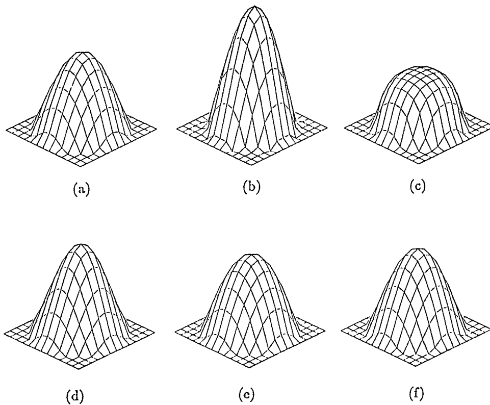
Figure 3.2. Reconstruction of a sinelike permittivity distribution with operating frequency at 10 MHz. The peak value of the relative permittivity is 11. The diameter of the object is one-tenth of the wavelength. (a) is the original distribution. (b) is the result of the first-order approximation. (c) to (e) are the results from the second iteration to the fourth iteration. (f) is the final convergent solution after five iterations.
