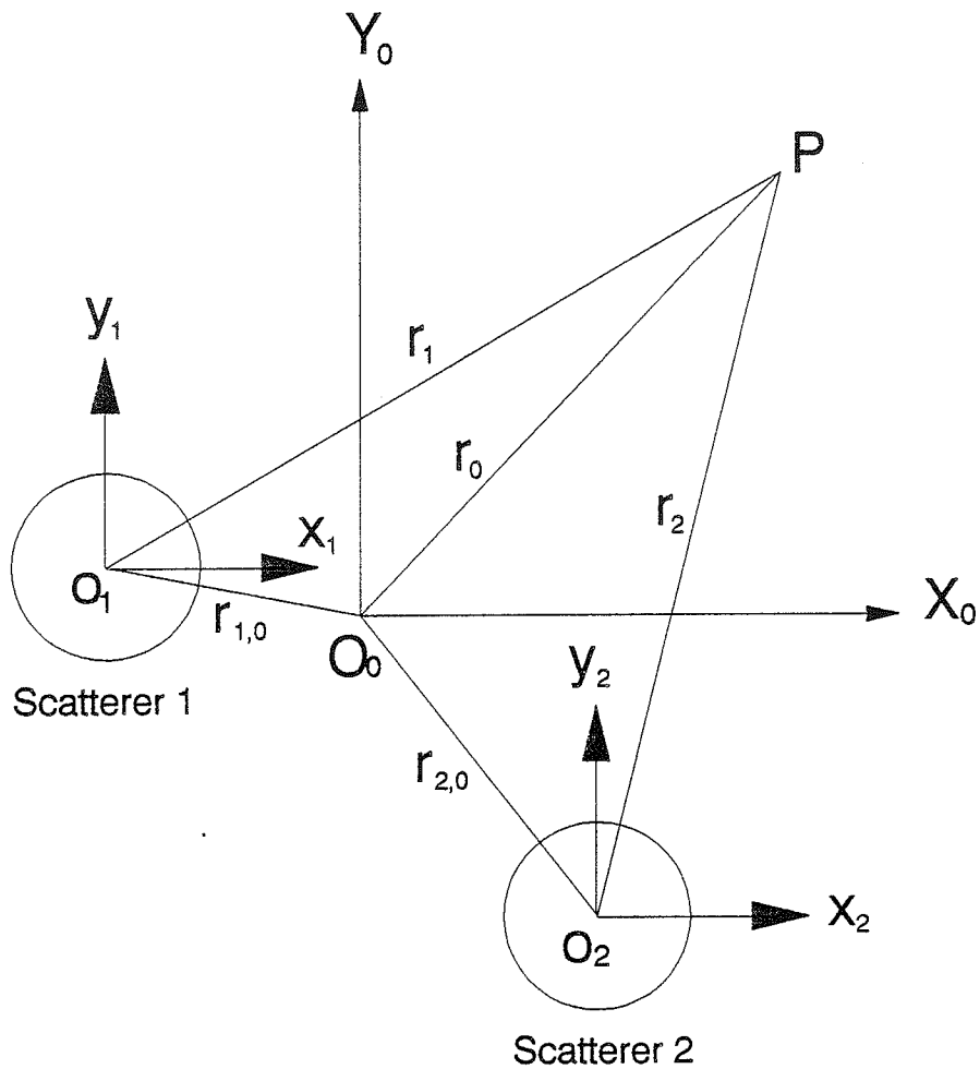
Figure 2.2. Coordinate systems of a two-scatterer problem. O_0 is the origin of the global coordinate system. O_1 and O_2 are the origins of the local coordinate systems related to the first and the second scatterers, respectively.
