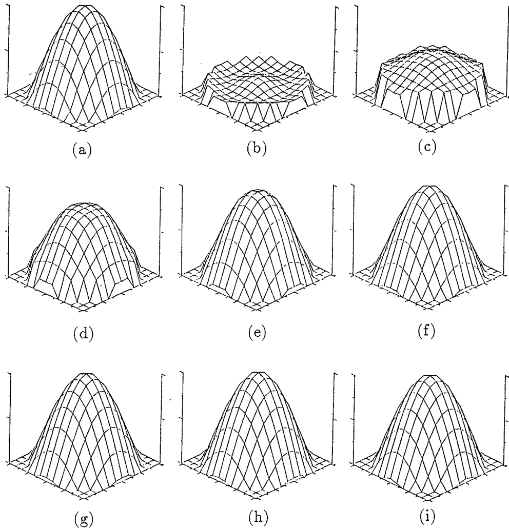
Figure 3.24. Evolution of the convergence of the real part of a complex permittivity distribution reconstructed by using the distorted Born iterative method with operating frequency at 100 MHz. The peak value of the real part of the relative permittivity is 2. The diameter of the object is 3.0 meters. (a) is the original distribution. (b) is the result of the first-order approximation. (c) to (h) are the results from the second iteration to the seventh iteration. (i) is the final convergent solution after twenty iterations.
