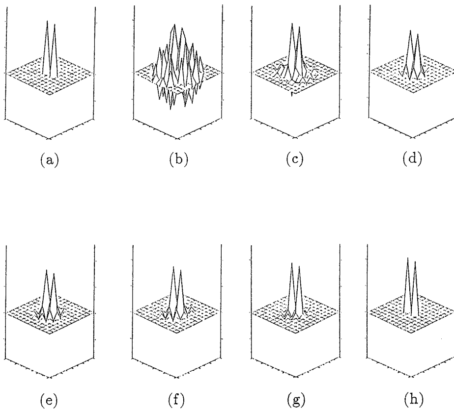
Figure 3.23. Reconstruction of a two single-pixel pulses separated by one pixel using the distorted Born iterative method with operating frequency at 100 MHz. The contrast of the relative permittivity is 1:2. The diameter of the reconstructed area is 3.0 meters. (a) is the original distribution. (b) is the result of the first-order approximation. (c) to (g) are the results from the second iteration to the seventh iteration. (h) is the final convergent solution after twenty iterations.
