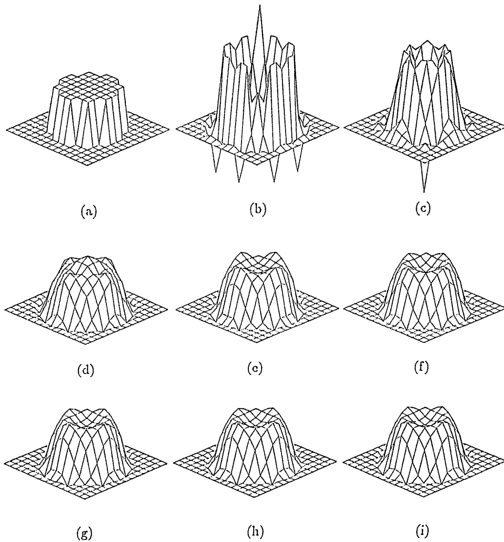
Figure 3.5. Reconstruction of a step permittivity distribution with operating frequency at 100 MHz. The contrast of the relative permittivity is 1:1.60. The diameter of the object is 1\lambda . (a) is the original distribution. (b) is the result of the first-order approximation. (c) to (h) are the results from the second iteration to the seventh iteration. (i) is the final convergent solution after eight iterations.
