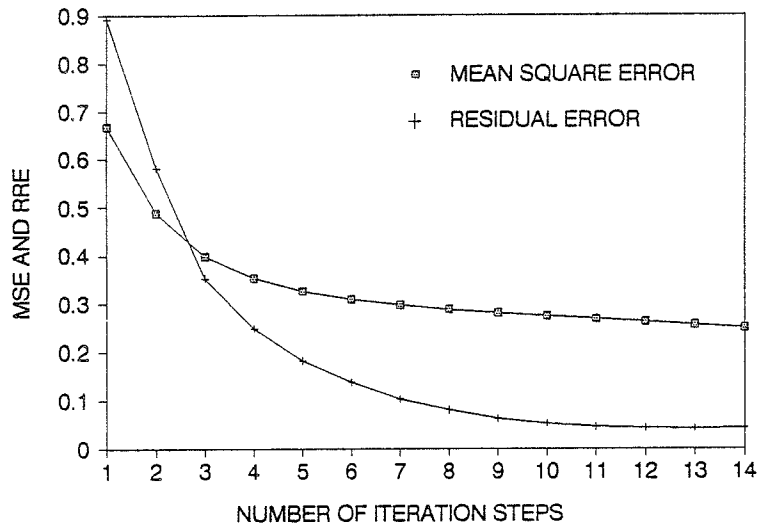
Figure 4.20. The relative MSE (Mean Square Error) and the RRE (Relative Residual Error) of the reconstructed permittivity distribution shown in Figure 4.18 as a function of the iteration steps.
