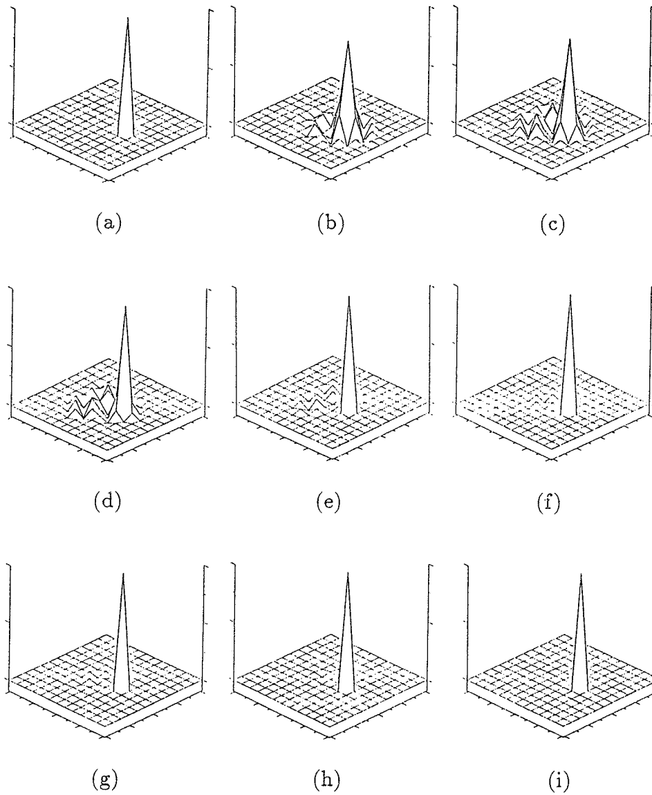
Figure 3.20. Reconstruction of a single-pixel pulse distribution by using the distorted Born iterative method with operating frequency at 100 MHz. The contrast of the relative permittivity is 1:2. The diameter of the reconstructed area is 3.0 meters. (a) is the original distribution. (b) is the result of the first-order approximation. (c) to (h) are the results from the second iteration to the seventh iteration. (i) is the final convergent solution after twenty iterations.
