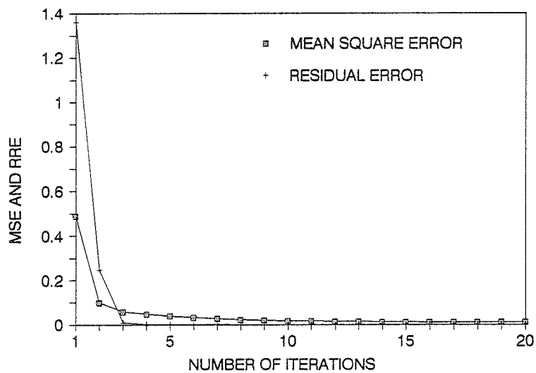
Figure 4.11. The relative MSE (Mean Square Error) and the RRE (Relative Residual Error) of the reconstructed permittivity distribution shown in Figure 4.9 as a function of the iteration steps.
